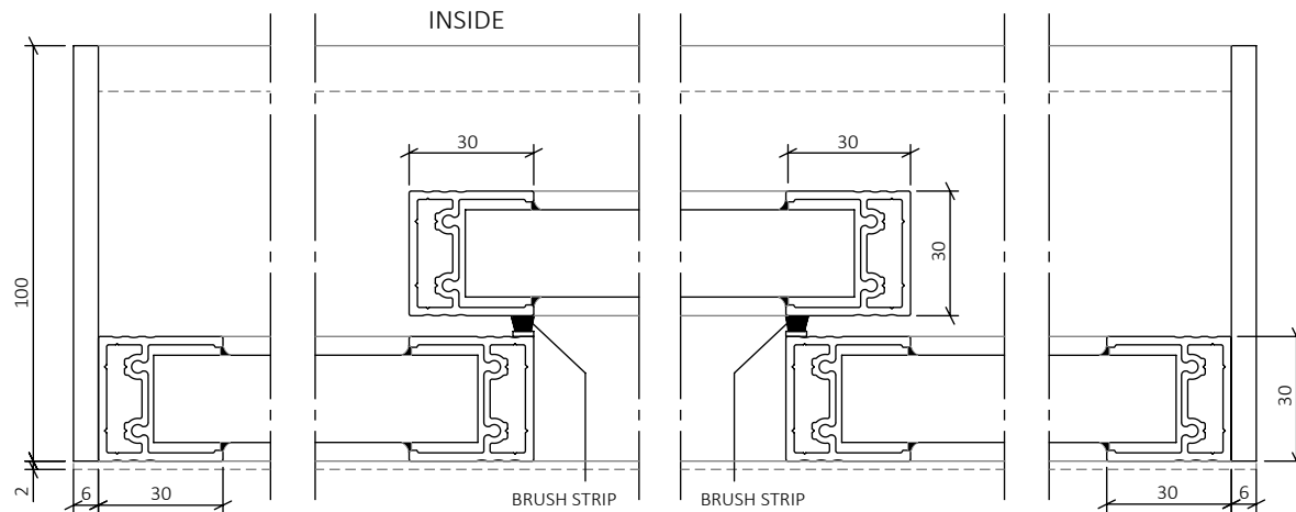
SECTION B-B SCALE 1:2
