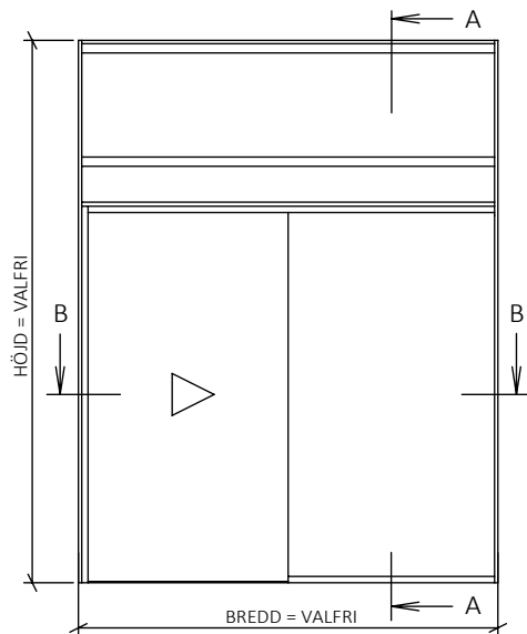
SCALE 1:20
