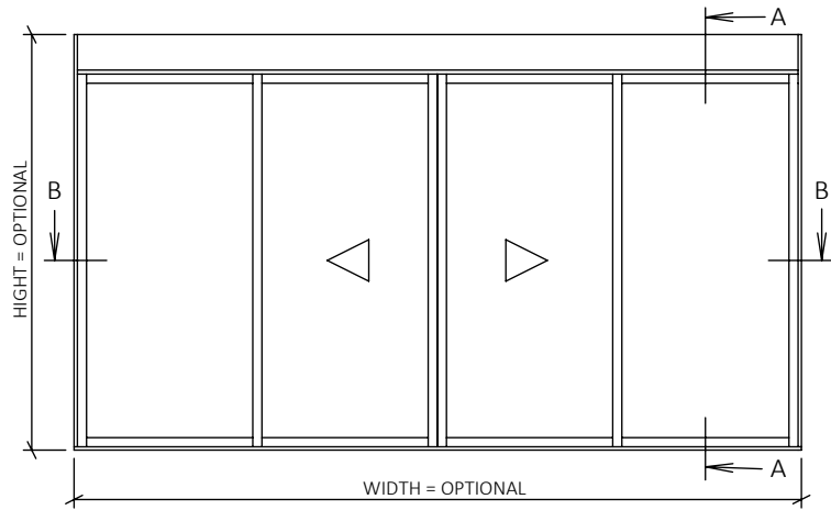
SCALE 1:20
