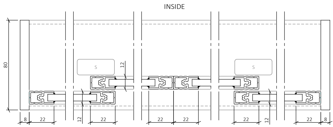
SECTION B-B SCALE 1:2
