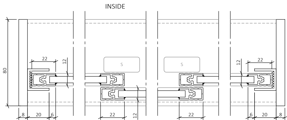
SECTION B-B SCALE 1:2
