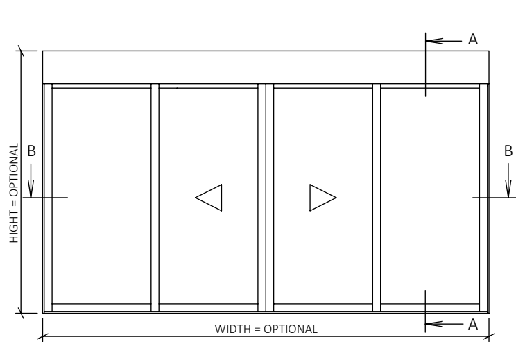
SCALE 1:20
